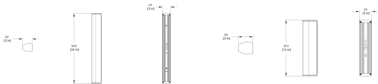
BRES-M Branch Sconce Medium Dimension
