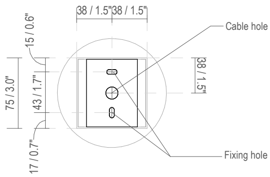
Fixing Dimensions
