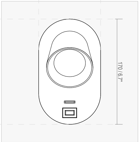
Fixing Dimensions
