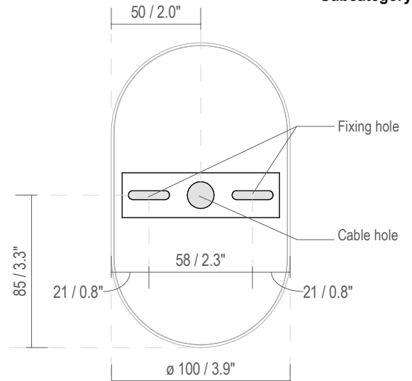
Fixing Dimensions
